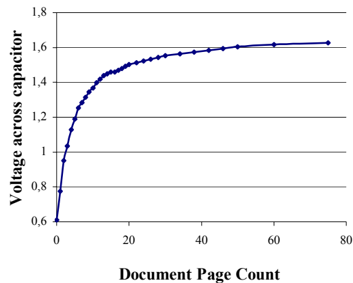
Figure 5. Measurement of pages in DigiClip
