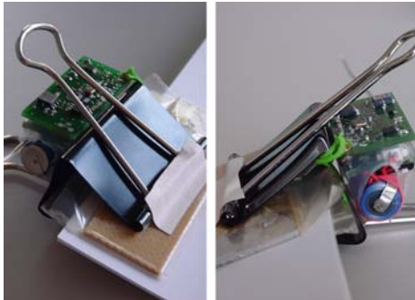
Figure 2. Close look at the DigiClip device.
