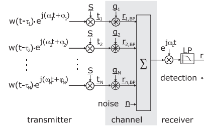
Fig. 3. Superimposed signals
