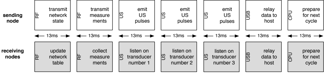
Figure 4: Relate dongles use a slotted protocol for data transmission over RF and ultrasonic sensing.
